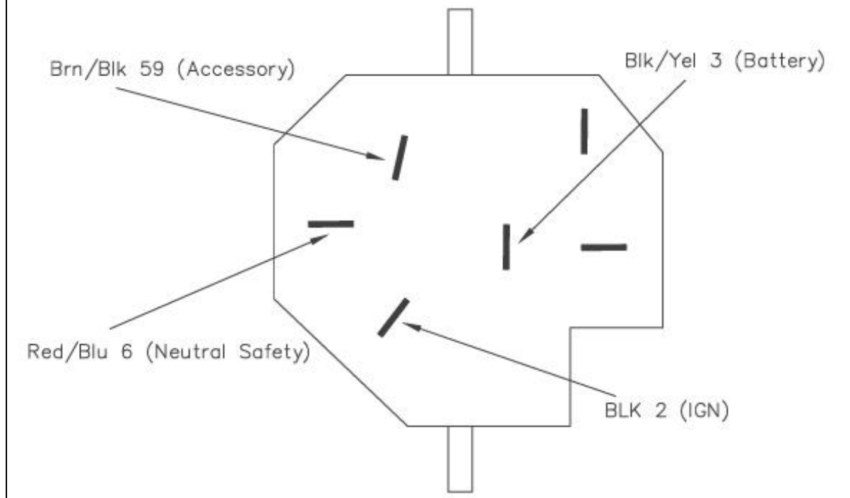
1977 Ford Truck Ignition Switch
