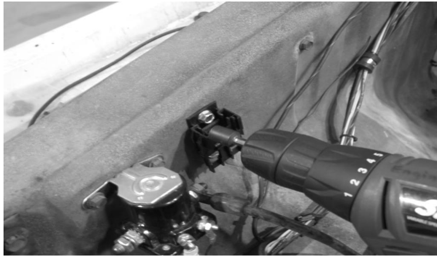
Figure 7-6 Installing the Maxi Fuse Holder '73-'77 Model
