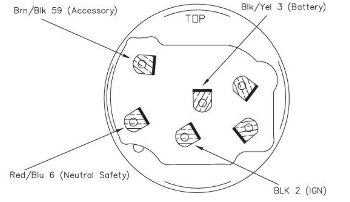
1970 – 1976 Ford Truck Ignition Switch
