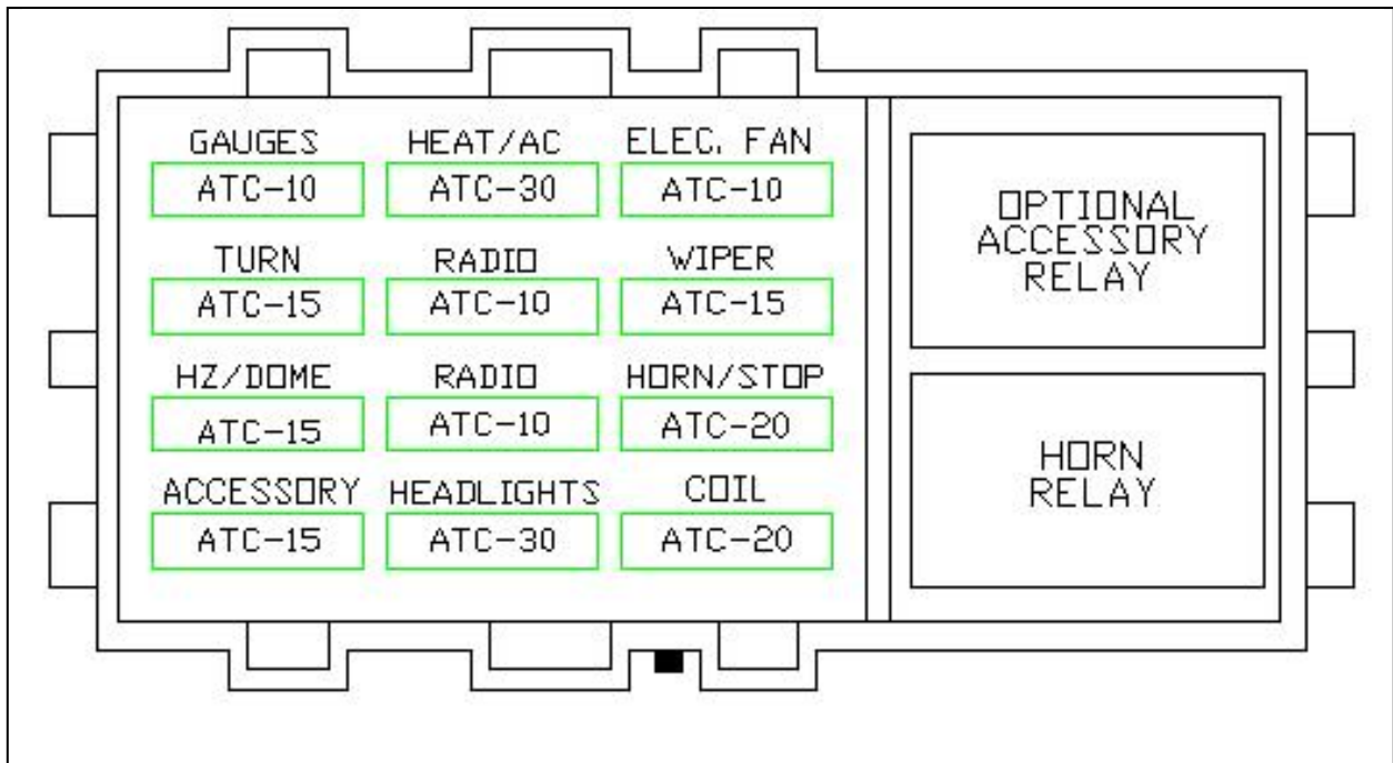
Figure 9.1 Fuse Requirements
