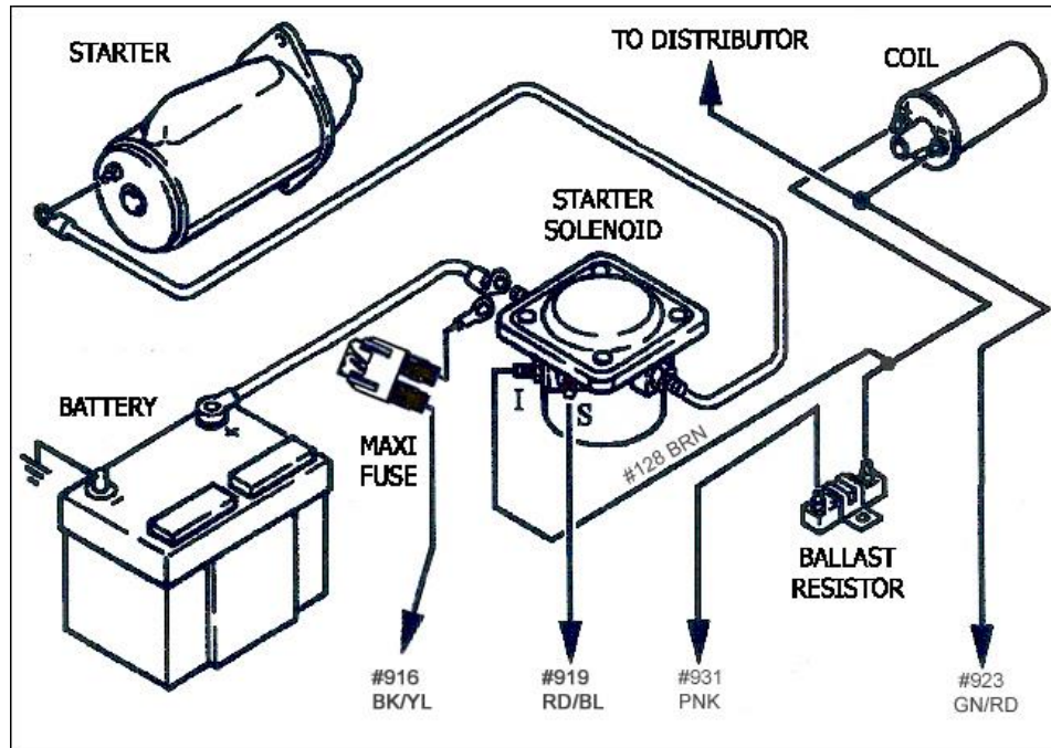
Figure 7-2A Ford Ignition (Start/Run) System
