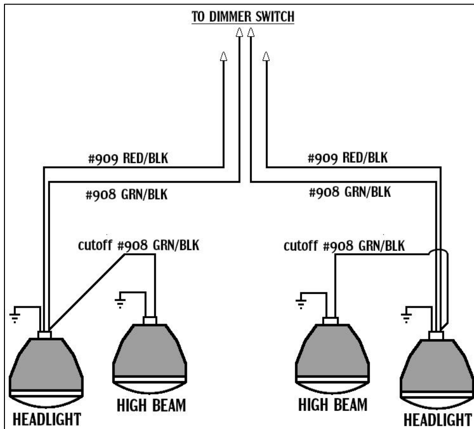
Figure 8.3B Dual Headlamp Connections
