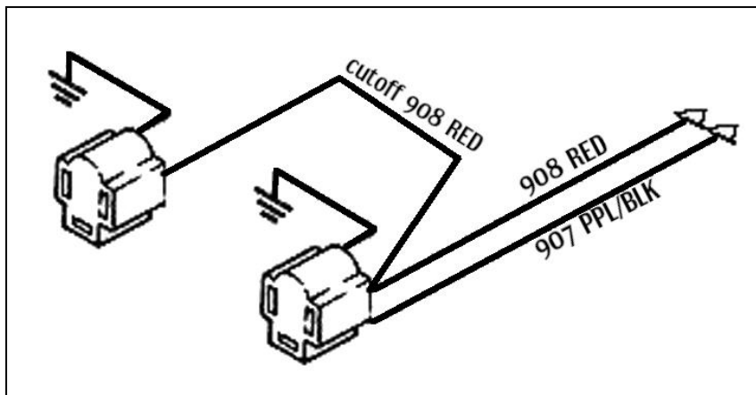
Figure 8.5A Dual Headlamp Connections
