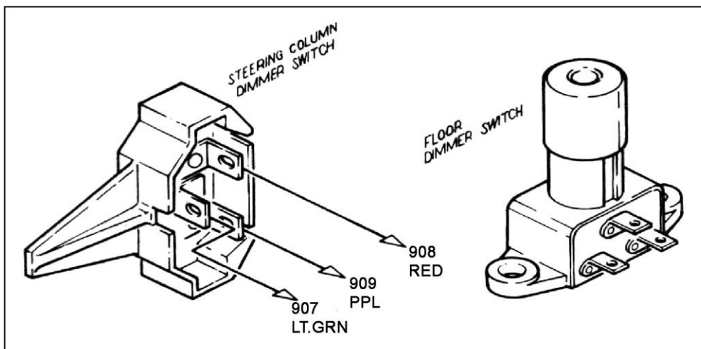
Figure 8-5B Dimmer Switches (Push Button Style – Painless Part #80150)
