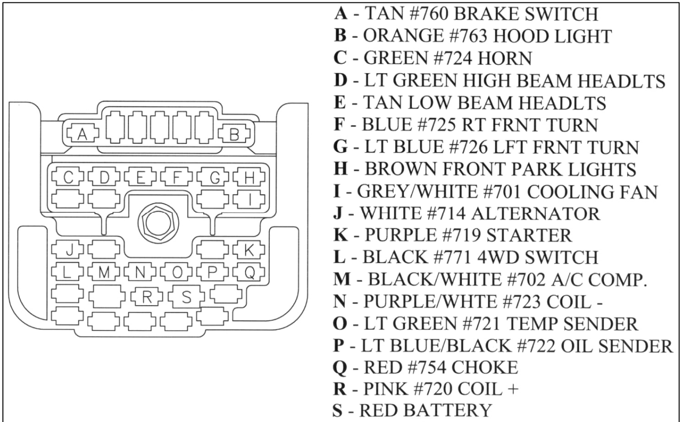
Illustration 3 Engine Harness Firewall Connector Style #2
