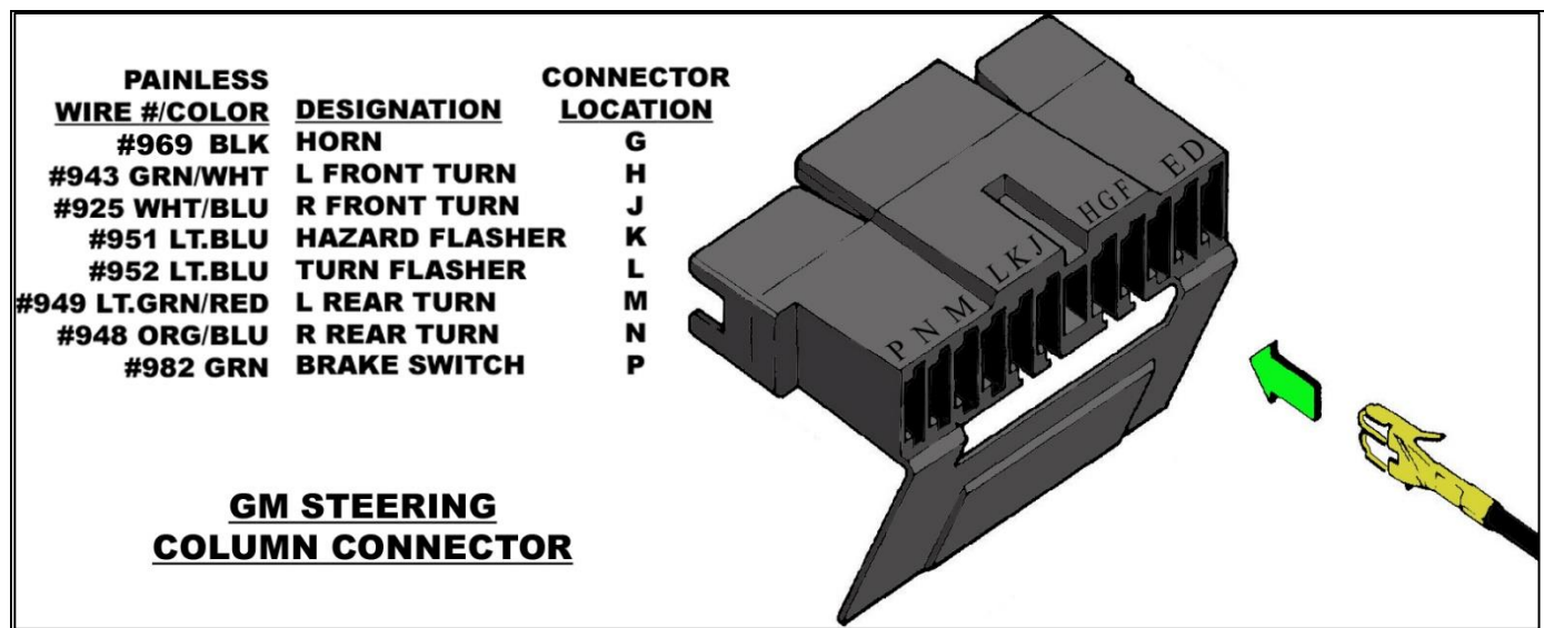
Figure 16 GM Steering Column Connector
