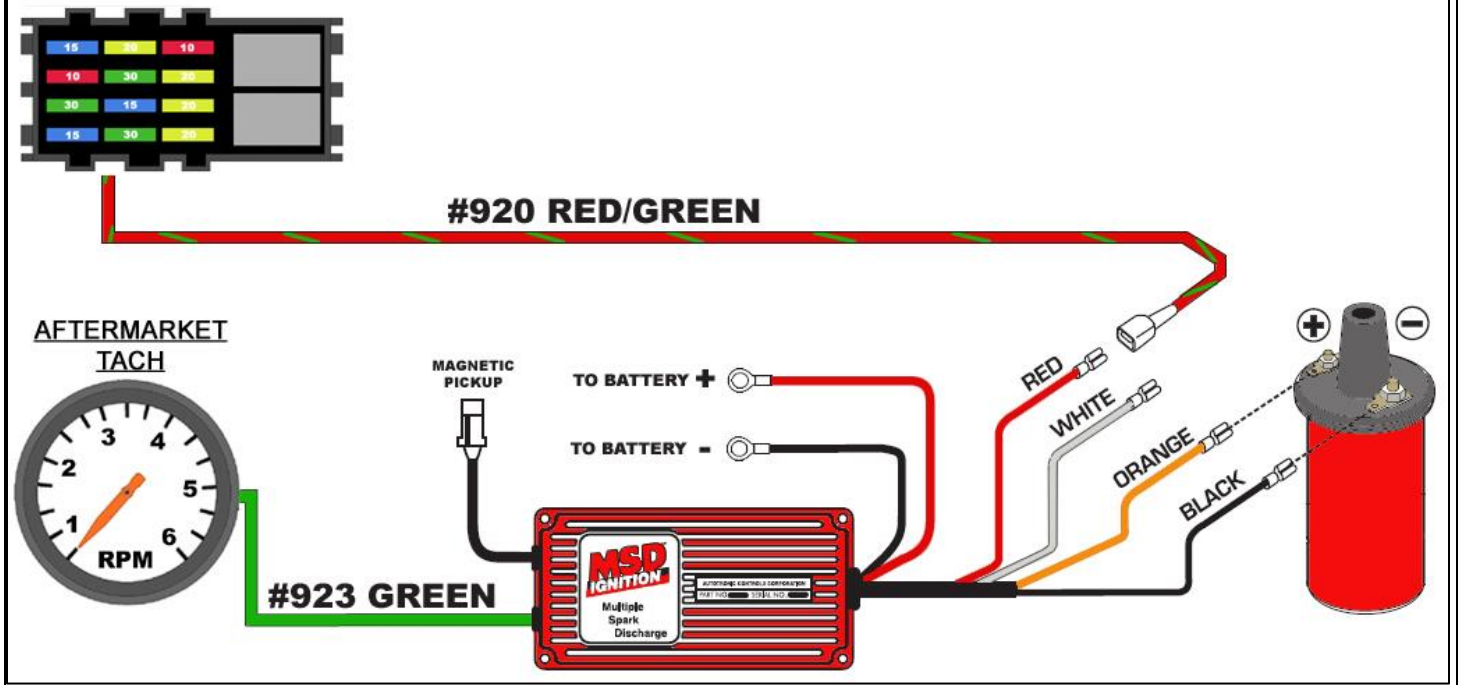
Figure 15 MSD Connections
