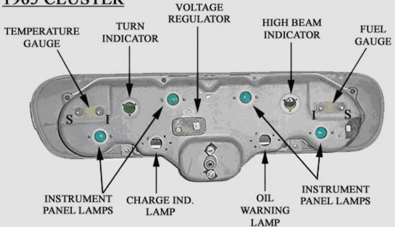
Figure 19 1965 Instrument Panel
