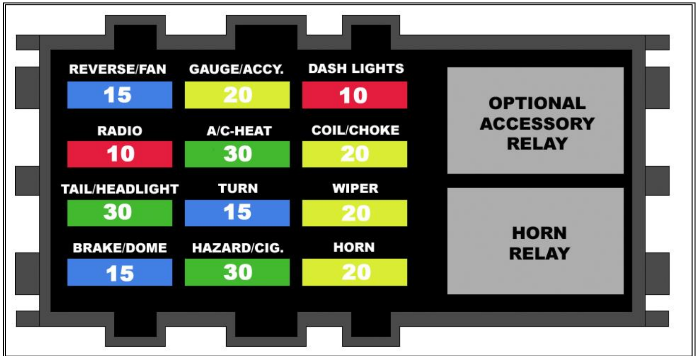
Figure 33 Fuse Requirements
