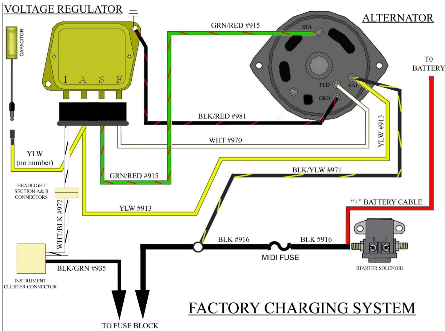
Figure 9 Ford Alternator
