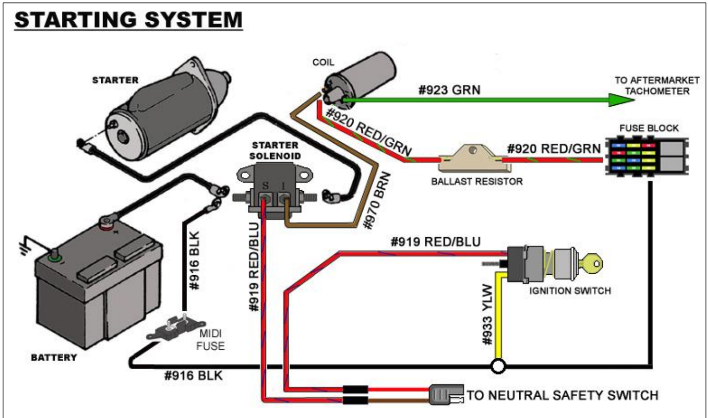
Figure 12 Ford Start/Run System
