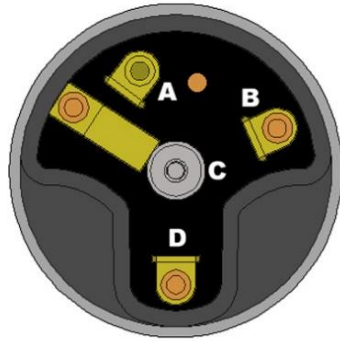
Figure 17 Ignition Switch Connections
