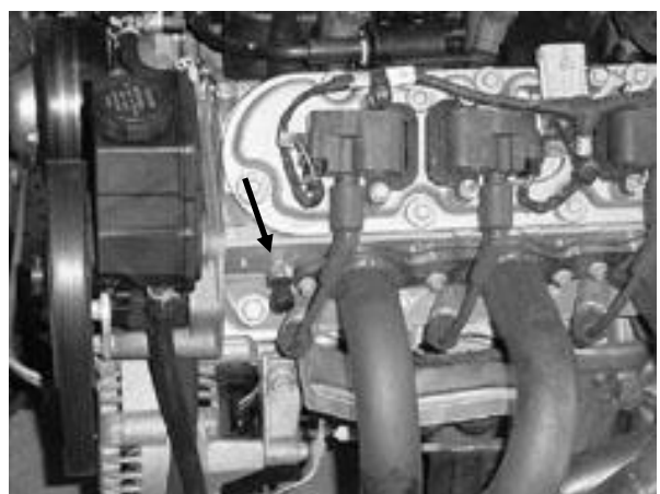
Figure 6.15 ECT Sensor
